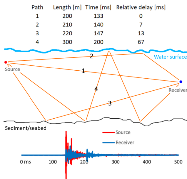
Figure 6. Boundary reflections lead to the signal being “stretched”, so the energy is spread temporally with the impulse losing its initial shape.
