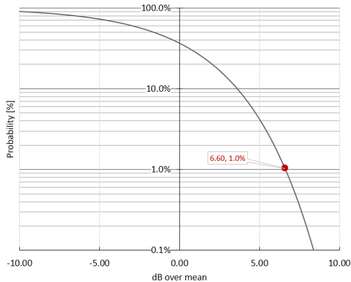
Figure 3. Plot of Eq. 6. Probability that a level is 'y' dB above the predicted mean level. Example call-out at suggested probability of exceedance of 1% (6.6 dB).
