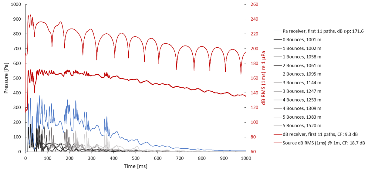
Figure 13. Example of tracking the first 11 paths from source to receiver (as straight lines, with perfect reflection at boundaries). Range 1000 m, depth 200 m, source depth 5 m, receiver depth 50 m. The source is a 4000 Cui seismic array (thin red line). Notice that the crest factor (CF \text{dB}_{zp} - \text{dB}_{RMS} ) is 18.7 dB at the source, but 9.3 dB at the receiver 1 km away (thick red line). Red lines read on right axis (dB), remaining lines on left axis (Pa).
