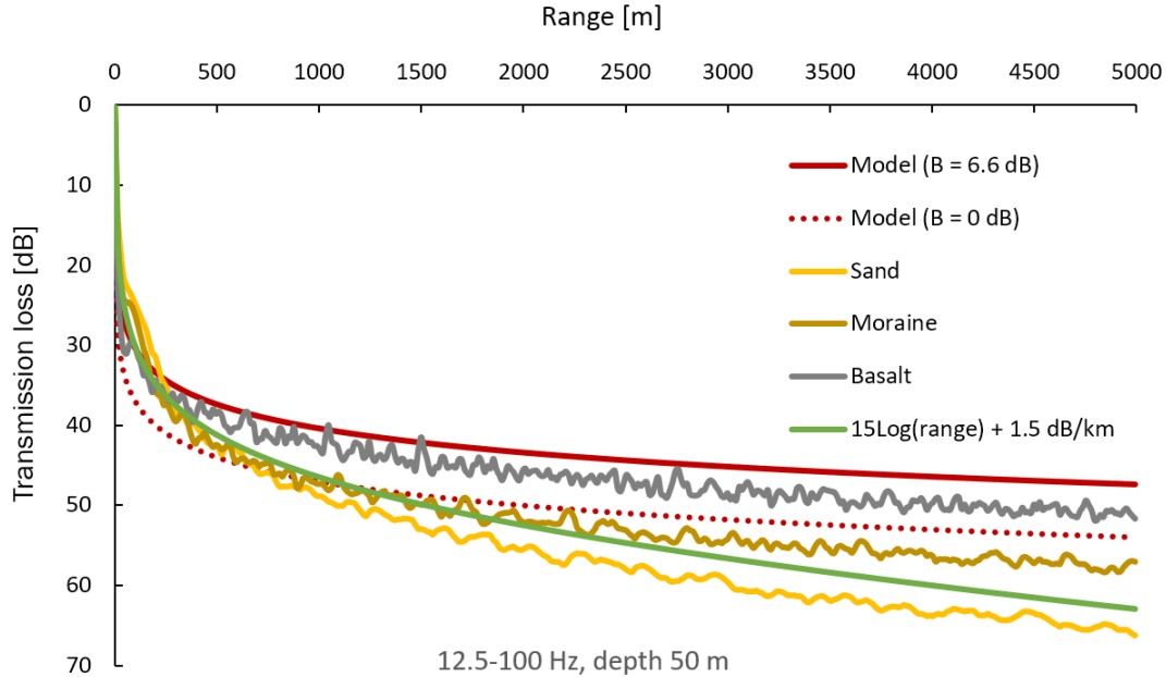
Figure 4. Effect of applying correction factor “B”. Modelling for data series “Basalt”, “Moraine” and “Sand” with dBSeaPE (Parabolic Equation method) to show effect of sediment as well as effect of changing “B”. Attenuation from absorption is ignored in this example due to the low frequencies modelled. Green line is example of a semi-spherical transmission loss with attenuation and channel leak estimated at 1.5 dB/km. The two series named “Model” are the model used in this framework with and without the correction term “B” applied.
