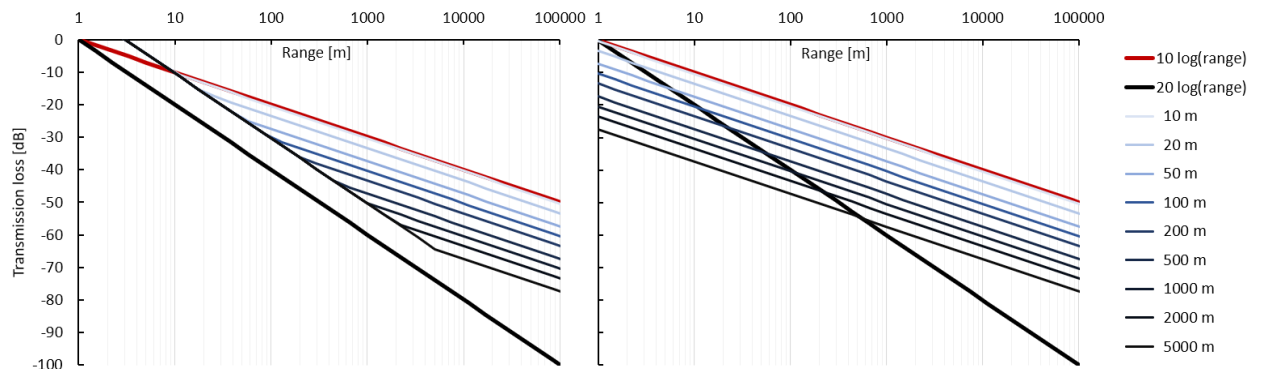
Figure 5. Comparison of transmission loss between adjusted (left) and non-adjusted model (right). For large depths the unadjusted model yields transmission losses larger than spherical spreading. The adjusted model predicts transmission losses equivalent to spherical spreading minus 10 dB until depth is larger than range.
